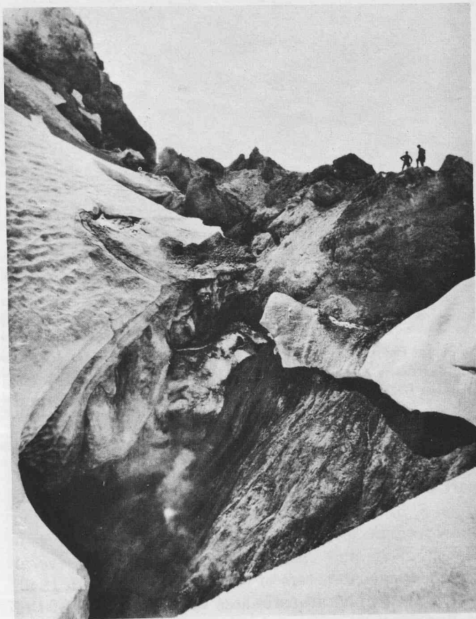
FIGURE 6. — Part of the west-rim thermal area, 1914. Photograph by Clyde Banks.
