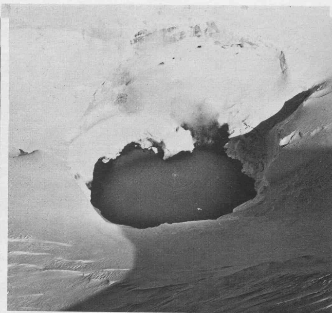
FIGURE 15. — Main area of upwelling within the crater lake. The lake was about 50 m across at this time, and the upwelling was about 2 m in diameter. Aerial photograph taken from the south, April 3, 1976.
