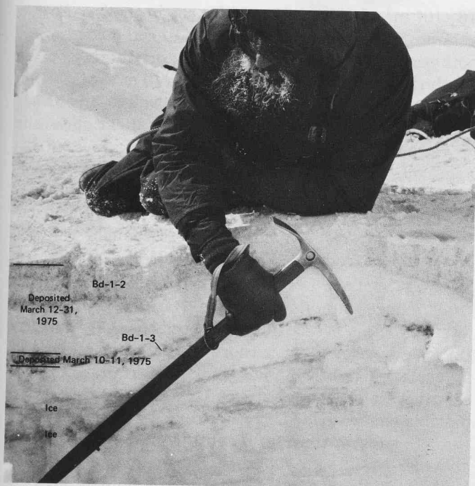
FIGURE 26. — Two layers of ejecta (samples Bd-1-2 and Bd-1-3, table 6) in crevasse wall 100 m west of the new main fumarole. Ejecta was being deposited on the snow surface at the time this photograph was taken, March 31, 1975.
