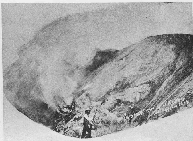
FIGURE 5. — Fumarole cluster on the west rim of Sherman Crater, 1909. Photograph by Henry Engberg.
