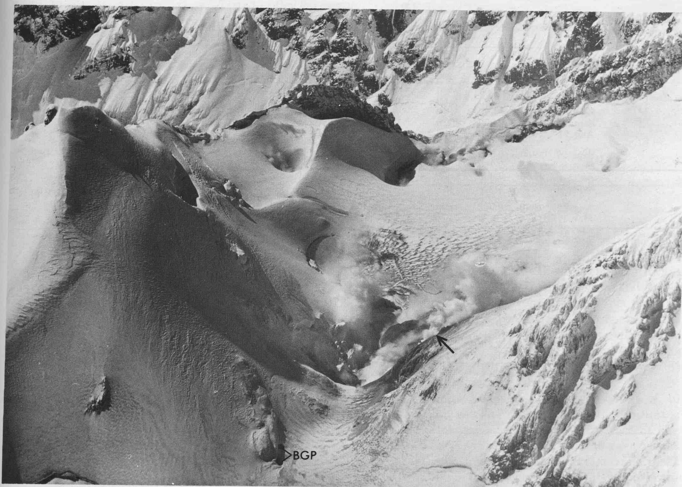
FIGURE 11. — Early westward view of increased thermal activity, March 27, 1975. Initial signs of new activity were the north pit (not shown), main fumarole (arrow), increased crevassing, and Boulder Glacier pits (BGP). For scale, the distance across the east breach from the top of Sherman Peak (upper left) to the top of Lahar Lookout (middle right) is about 500 m. Aerial photograph by Austin Post.
