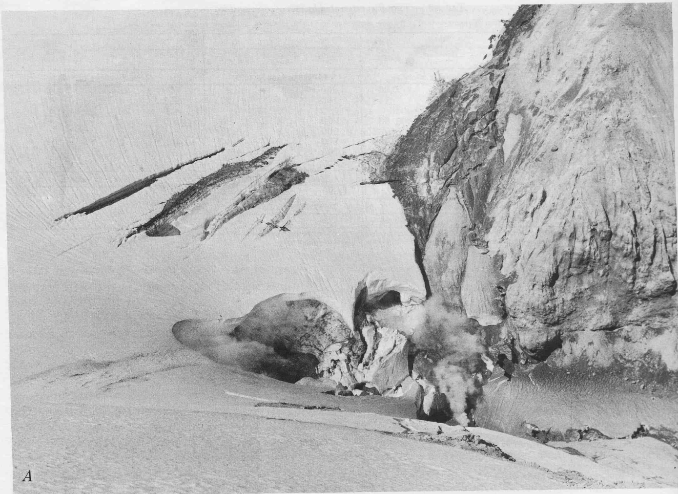
FIGURE 12. — View from Sherman Peak of the site of the new main fumarole at the south base of Lahar Lookout. A, August 17, 1974, the two clusters of activity are evident near the east breach, including a prominent plume from the old main fumarole. B, July 6, 1975, a dense particle-laden plume extends from the 1- × 5-m opening of the new main fumarole, which occurs on a rock rib that had no sign of vapor
