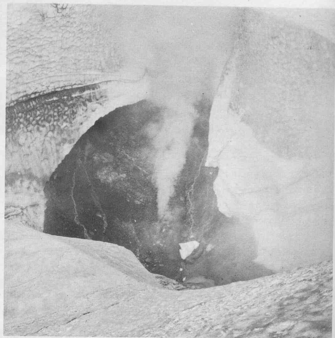
FIGURE 16. — Highly pressurized high-pitched fumarole in the southwest pit (SWP), July 16, 1975. The fumarole opening is about 15 cm wide, and the ice pit is about 20 m wide, from left to right.
