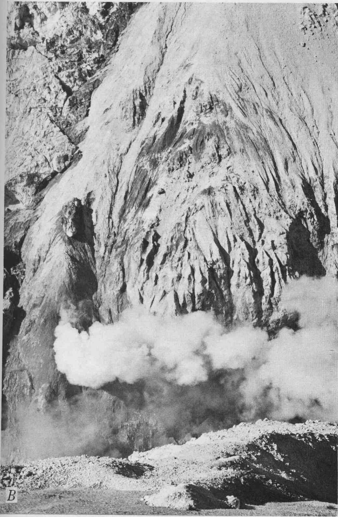
emission in 1974. C, February 6, 1976, vapor still issues from this fumarole, but without ejecta. The snowmelt pattern delineates the area of thermal ground around the fumarole.
