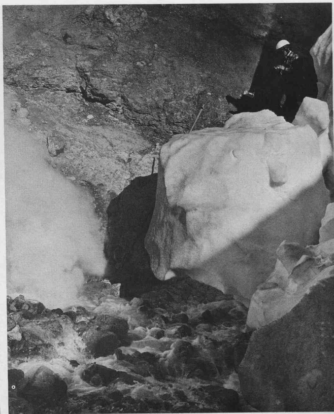
FIGURE 7. — Northward view of the old main fumarole near the east breach of Sherman Crater, August 16, 1974. This fumarole lies at the south base of Lahar Lookout.
